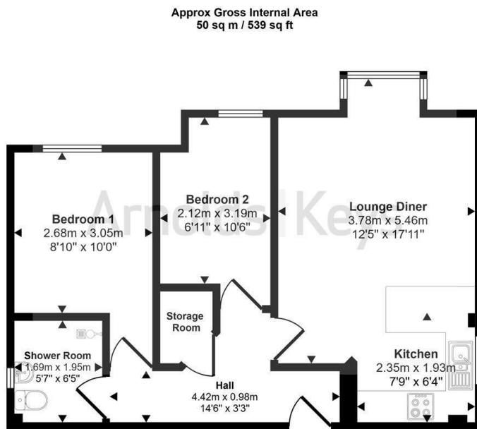
Floorplan
