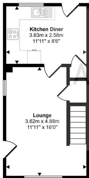
Ground Floor Approx 28 sq m / 297 sq ft
