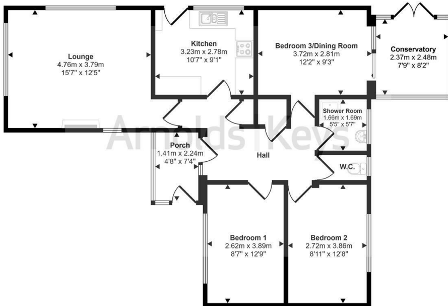
Floorplan
