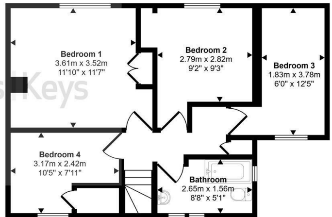
First Floor Approx 50 sq m / 543 sq ft
